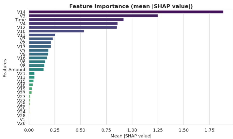
Figure 4. Interpreting the Logistic Regression Model: SHAP Value Analysis for Feature Importance Source: Research Findings
