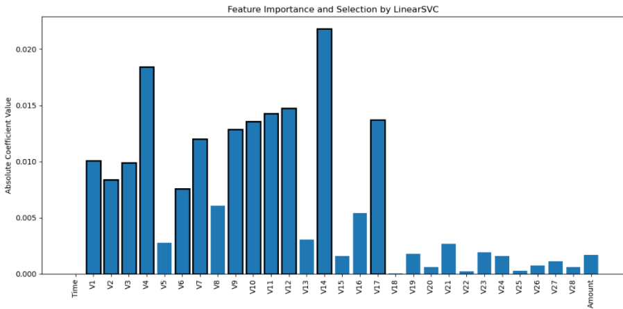
Figure 3. Feature Importance and Selection by LinearSVC
