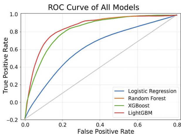
Figure 1. ROC Curves for All Models
