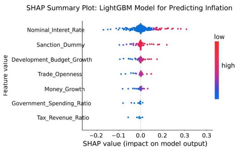
Figure 4. SHAP summary plot for the LightGBM inflation model Source: Research findings
