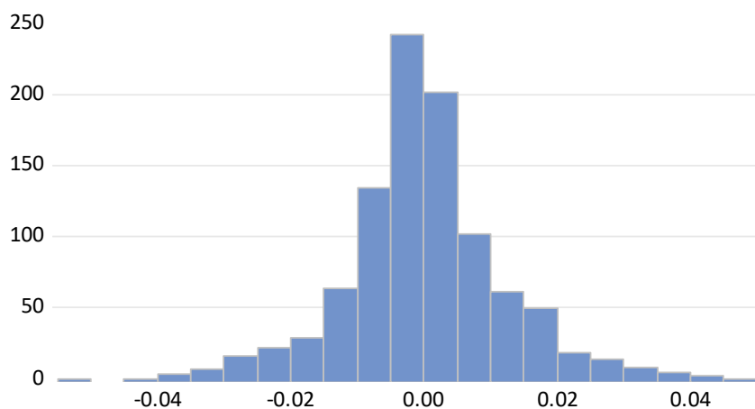
Figure 3. Residual normality test of OLS estimation
