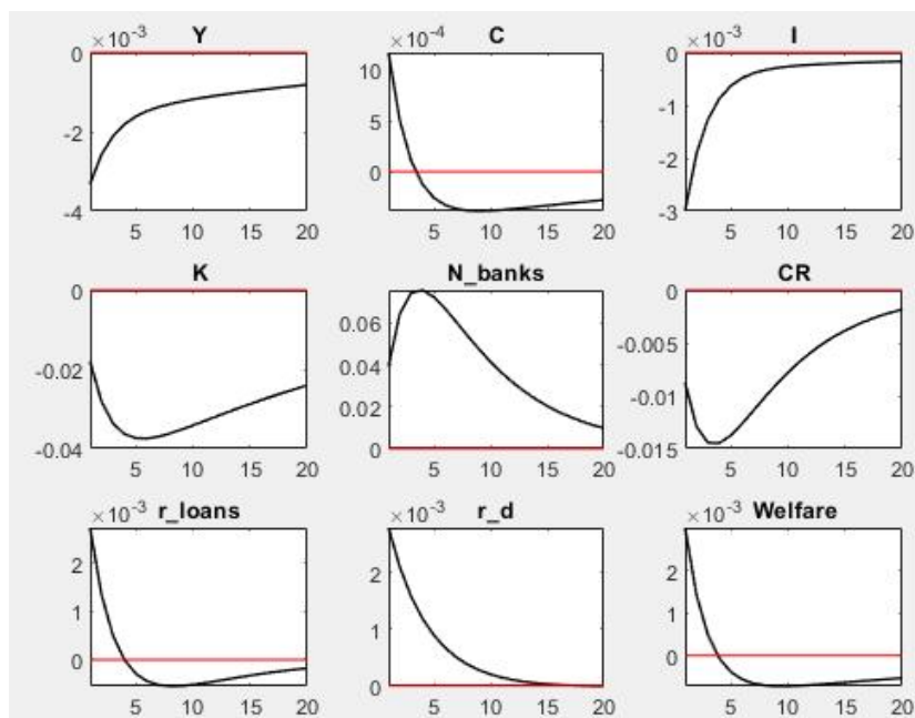
Figure 3. Impulse Response Functions (IRFs) of Liquidity Shock
