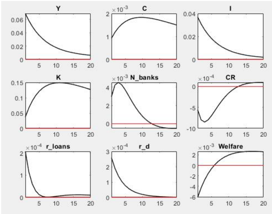
Figure 2. Impulse Response Functions (IRFs) of Productivity Shock Source: Research Findings
