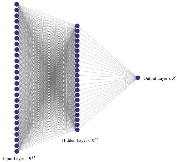
Figure 8. Architecture of the MLP Model for Data Simulation and Prediction. Source: Research findings
