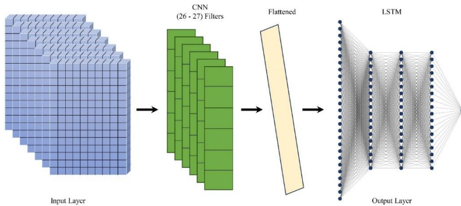
Figure 7. Architecture of the Hybrid CNN-LSTM Model for Data Simulation and Prediction.
