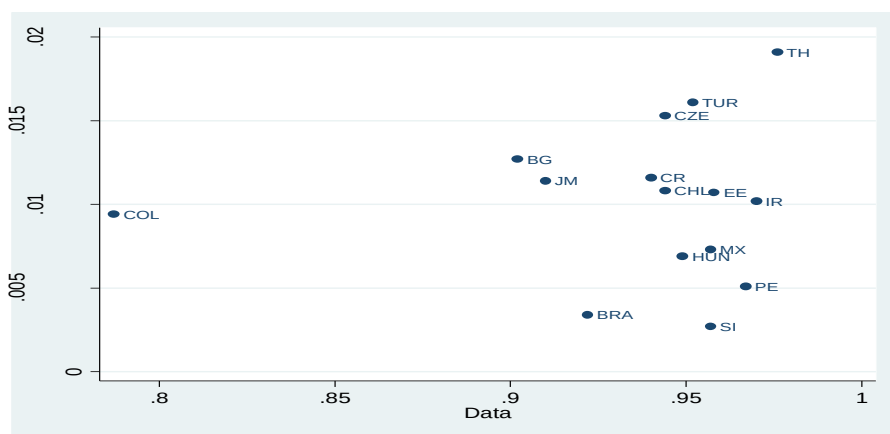
Figure 11. Vacancies auto-correlation
