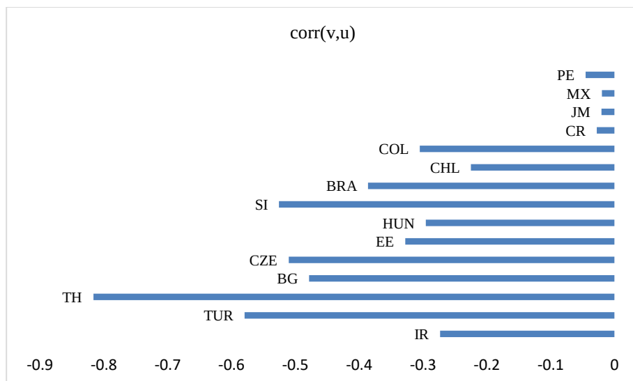
Figure 5. Vacancies-unemployment correlation
