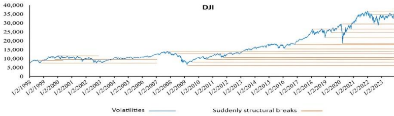
Figure 3. Structural Breaks in the Time Path of the Dow Jones Index
