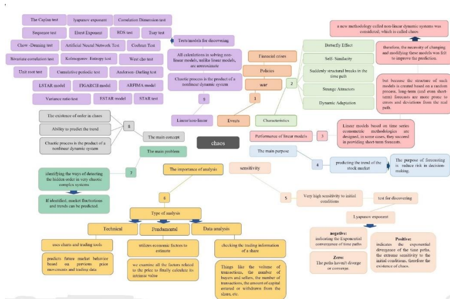
Figure 4. A Conceptual Chaos Model for Financial Markets Source: Research findings
