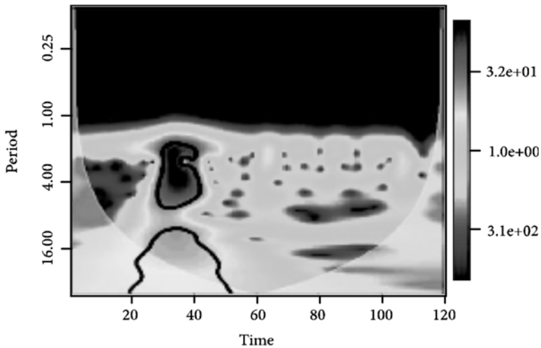
Figure 3. The Energy Power Spectrum for Financial Stability Index. Source: Research findings.
