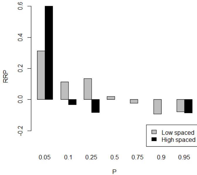
Figure 3. Loss Domain.
