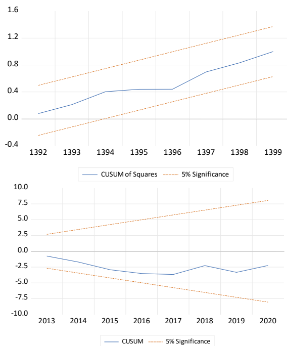
Figure 6. CUSUM and CUSUMSQ series for ARDL model and AIC.
