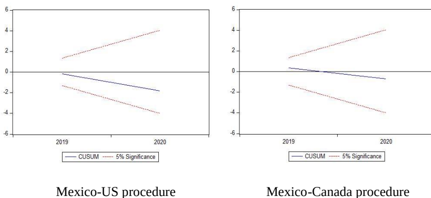
Figure 2. CUSUM results for scenario 1. Mexico trade deficit
